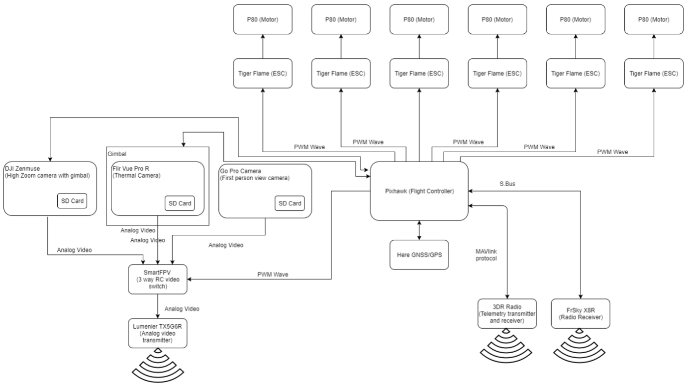
Figure 2.1.2: Onboard Hardware Layout
