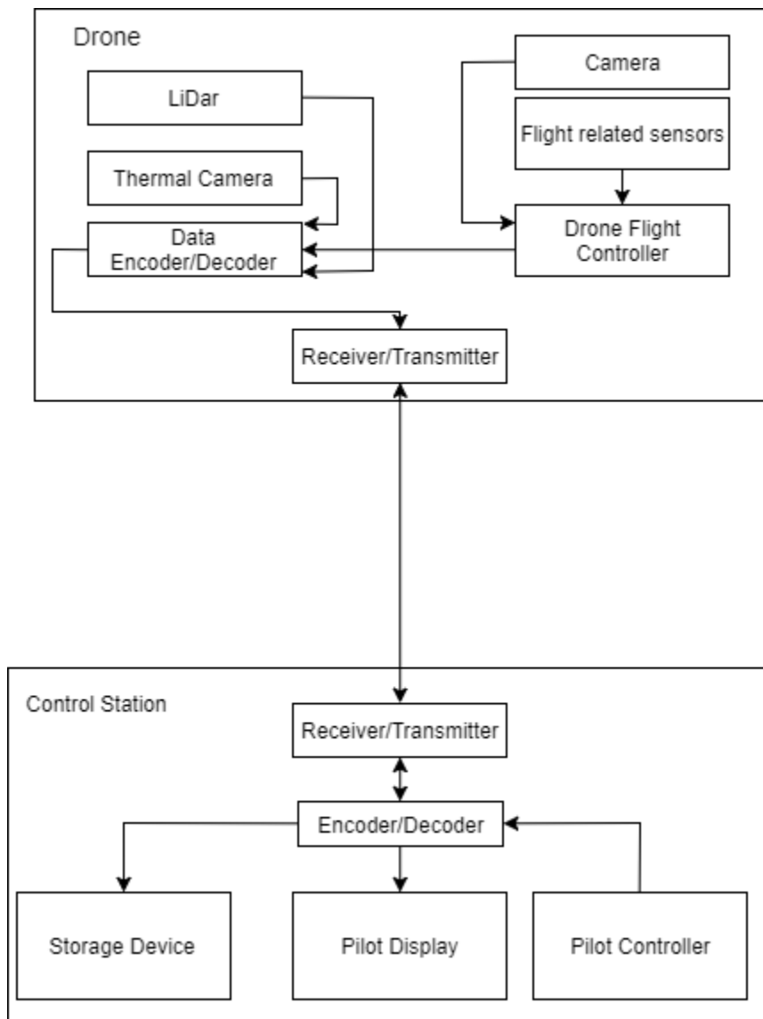
Figure 2.o.4: Single Transmitter
